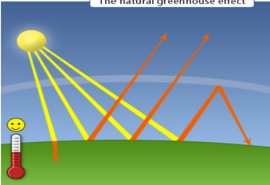
The natural greenhouse effect
